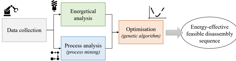
Fig. 1. Framework proposal for energy-effective DSP.
