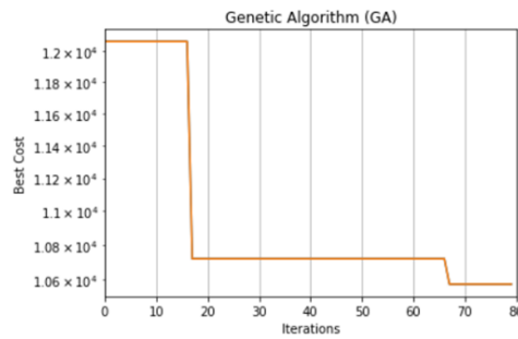
Fig. 5. GA fitness function value by iteration for the simulated scenario.
