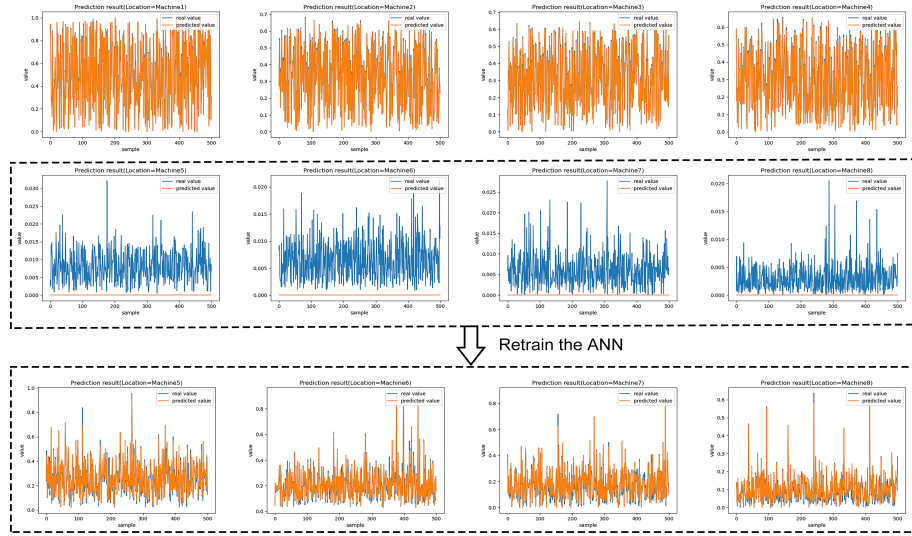
Fig. 3. ORCT Prediction results at different machines.
