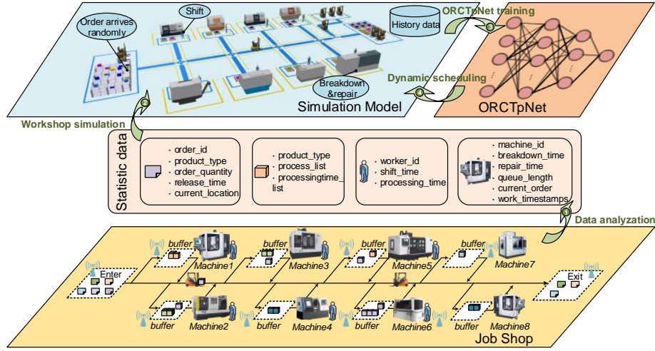
Fig. 1. Framework of dynamic scheduling with online predicted ORCT.
