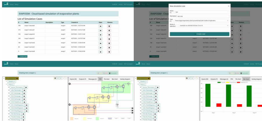
Fig. 3. Top-left: start page of the EVAPOSIM web-app; Top-right: new case creation form of the EVAPOSIM web-app; Bottom-left: case detail page of the EVAPOSIM web-app with PFD view; Bottom-right: case detail page of the EVAPOSIM web-app with bar chart view.
