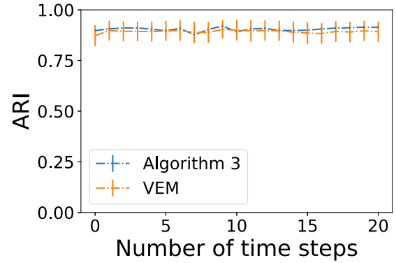
(a) P_{11} = 0.2
