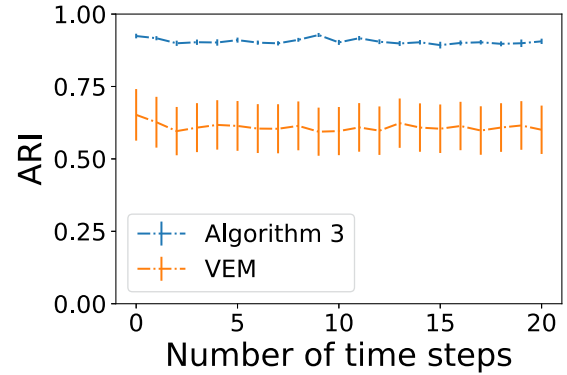
(b) P_{11} = 0.5
