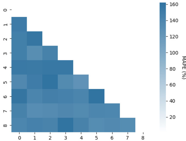
Fig. 6: Topogoly A: Testing NN on all node pairs combinations
