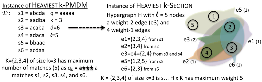
Fig. 2 An example of the reduction from HEAVIEST k -PMDM to HEAVIEST k -SECTION. The solutions are at the bottom. Each edge has its weight in brackets and the total weight is d = 6
