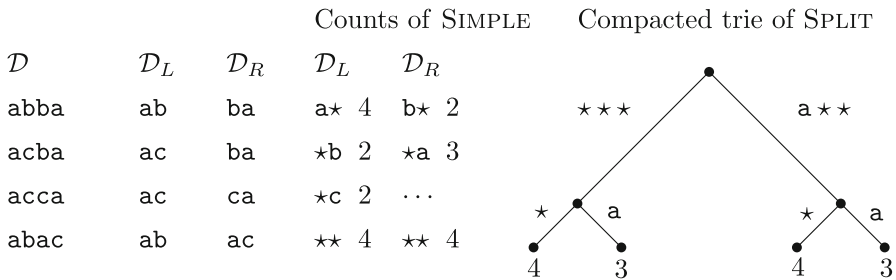
Fig. 3 Let \tau = 3 . If both q'_L and q'_R are 3-frequent (we check this using the counts of DS SIMPLE), then we read the count for q'_L q'_R from the compacted trie of DS SPLIT. If q'_L is 3-infrequent, then we apply SMALL- \ell on q_R and on the dictionary consisting of at most \tau = 3 strings from \mathcal{D}_R corresponding to the right halves of strings in \mathcal{D}_L that match q'_L
