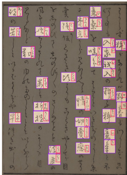
Ground truth
