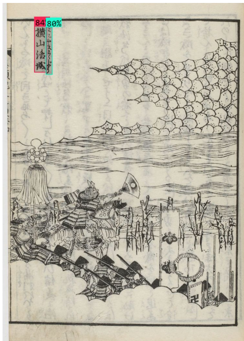
Prediction
