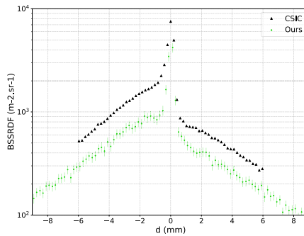
Fig. 15. Validation of the BSSRDF measurements performed on sample S9 from [9], at 550 nm, for \theta_i = 45^\circ, \phi_i = 0^\circ, \theta_o = 0, \phi_o = 180^\circ . The profile obtained with our device (green round dots) are compared with the profiles from [9] obtained with the device from CSIC (black triangle dots). Our device allows to measure the BSSRDF up to \pm 4 cm away from the incident spot. To the width of the CSIC profiles, our results matches the one from CSIC with a nearly constant offset.
