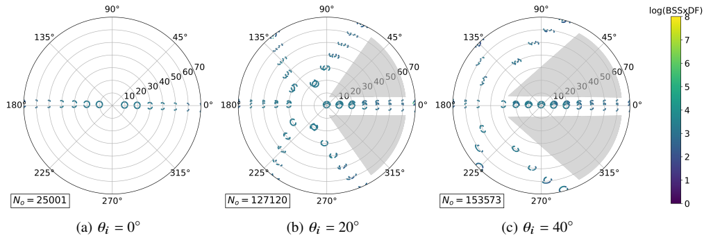
Fig. 14. Angular distribution ( \theta_r, \Delta\phi = |\phi_i - \phi_r| ) of the measurements performed at 550 nm in reflection on alabaster for a given incidence \theta_i and for a given range of distances from the illumination spot d_r = |\mathbf{x}_i - \mathbf{x}_r| \in [2, 2.1 \text{ cm}] . Each plotted point represents one BSSRDF measurement. The total number of valid measurements after data processing (cf. Sec. 6.3) is displayed as N_o . Because of the ambiguity on \phi_i at normal incidence, only nearly in plane measurements can be performed. Out of plane measurements are obtained while increasing the incidence. For grazier incidences, some domain of the reflective hemisphere remains completely ignored (gray areas).
