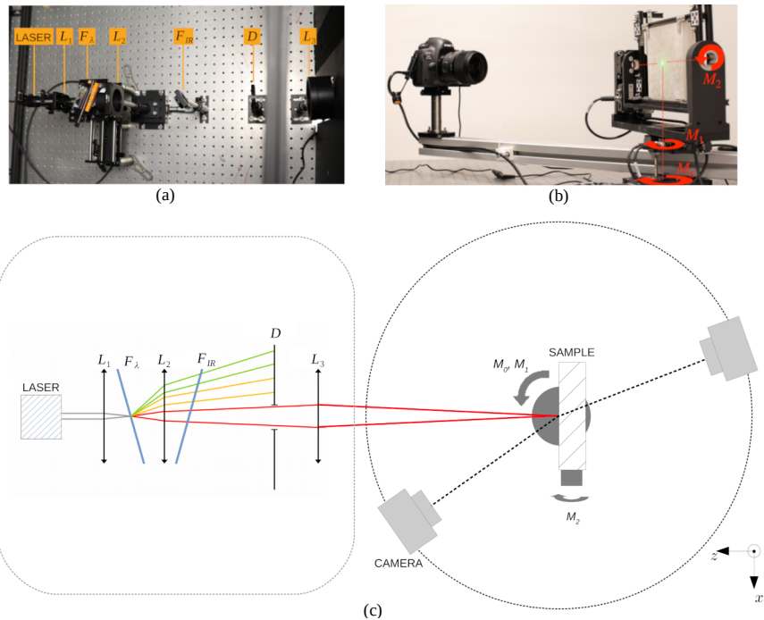
Fig. 2. Optical design of our setup for BSSxDF measurement. (a) The white laser beam is spectrally filtered by a continuously variable bandpass filter F_{\lambda} , and focused onto the sample's surface. (b) A camera collects the light scattered by the sample in multiple incidence/observation geometries by rotating the three rotation stages M_0 , M_1 , and M_2 . The camera is rotated using M_0 to reach various observation directions. M_1 and M_2 control the rotation of the sample around two different axes depicted by the red dotted lines, allowing the illumination direction to be varied as well. (c) Schematic representation of the device. Both BSSRDF and BSSTDF can be measured by positioning the camera either in front of or behind the sample.
