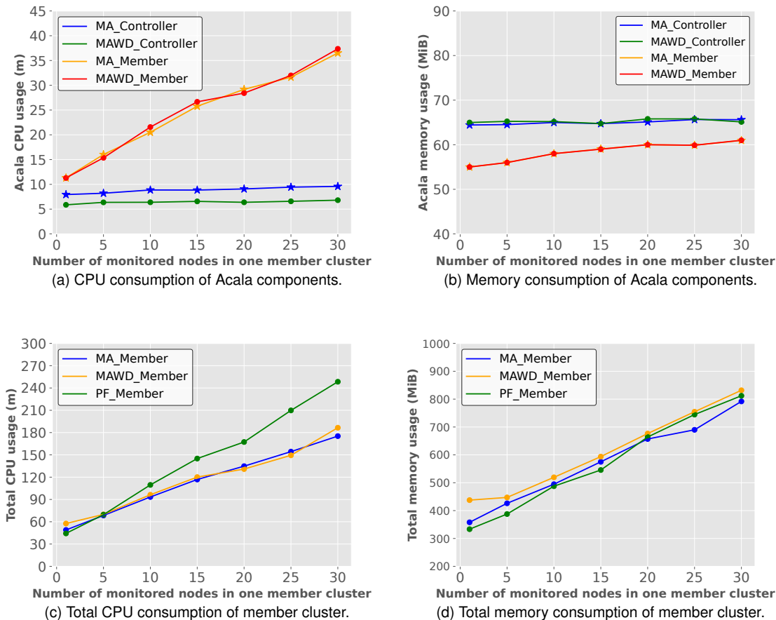
Fig. 8. CPU (a) and memory (b) consumption of Acala components and total CPU (c) and memory usage (d) of member cluster when scrape interval is set to 5 seconds.
