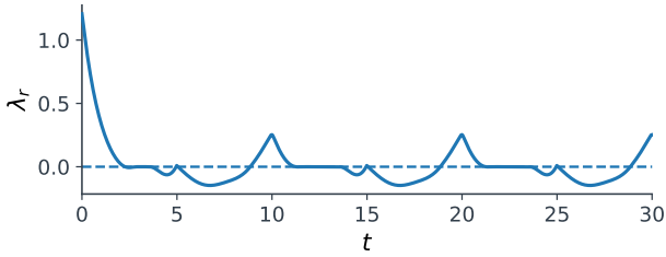
(b) Time plot of \lambda_r . The sign of this adjoint variable determines the value of \alpha_{opt} . The intervals on which \lambda_r is zero correspond to the singular arcs of \alpha_{opt} .
