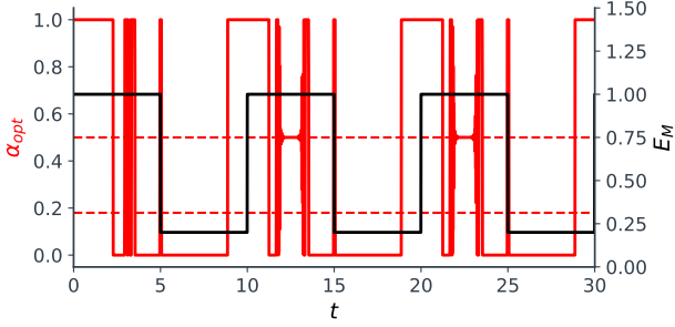
(a) The optimal control. The top dotted line corresponds to \alpha_{opt}^*(E_M^{\max}) and the bottom one to \alpha_{opt}^*(E_M^{\min}) .
