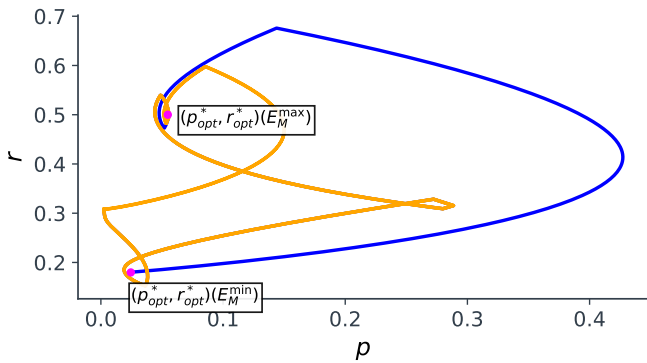
Figure 3: Phase plot of the variables p and r from (1), on the time-interval [0, 3T] and under \alpha_{opt} . In blue, over the first period and in orange over the second and third periods. The solutions of the static OCP corresponding to both possible values of E_M are highlighted.
