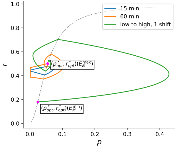
Figure 10: Different limit cycles of the system under the on-off control corresponding to different values of the environmental period T . The dotted line corresponds to r = g(p) , the switch in \alpha . The equilibrium points corresponding to E_M^{\max} and E_M^{\min} are also marked.
