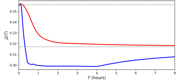
Figure 6: Average growth rate on a period of the limit cycle, under the optimal \alpha (red) and the on-off control (blue). The top dotted line corresponds to \mu_{avg}^* and the bottom one to \mu_J .
