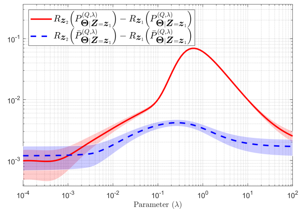
Fig. 5. Average of the differences R_{\mathbf{z}_2}(P_{\Theta|\mathbf{Z}=\mathbf{z}_1}^{(Q,\lambda)}) - R_{\mathbf{z}_1}(P_{\Theta|\mathbf{Z}=\mathbf{z}_1}^{(Q,\lambda)}) and R_{\mathbf{z}_2}(\bar{P}_{\Theta|\mathbf{Z}=\mathbf{z}_1}^{(Q,\lambda)}) - R_{\mathbf{z}_1}(\bar{P}_{\Theta|\mathbf{Z}=\mathbf{z}_1}^{(Q,\lambda)}) , with the measures P_{\Theta|\mathbf{Z}=\mathbf{z}_1}^{(Q,\lambda)} and \bar{P}_{\Theta|\mathbf{Z}=\mathbf{z}_1}^{(Q,\lambda)} in (10) and (16), respectively, computed over one hundred different training and test dataset random selections.
