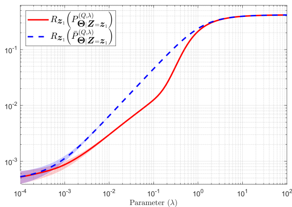
Fig. 3. Average Training Error: average of the expected empirical risks R_{\mathbf{z}_1}(P_{\Theta|\mathbf{Z}=\mathbf{z}_1}^{(Q,\lambda)}) and R_{\mathbf{z}_1}(\bar{P}_{\Theta|\mathbf{Z}=\mathbf{z}_1}^{(Q,\lambda)}) , with the measures P_{\Theta|\mathbf{Z}=\mathbf{z}_1}^{(Q,\lambda)} and \bar{P}_{\Theta|\mathbf{Z}=\mathbf{z}_1}^{(Q,\lambda)} in (10) and (16), respectively, computed over one hundred different training and test dataset random selections.
