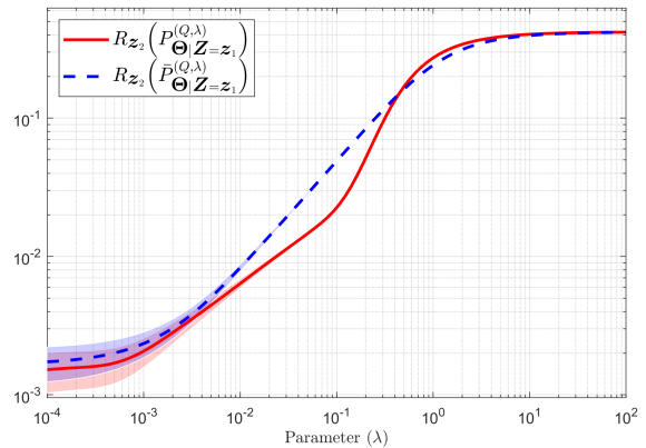
Fig. 4. Average Test Error: average of the expected empirical risks R_{\mathbf{z}_2}(P_{\Theta|\mathbf{Z}=\mathbf{z}_1}^{(Q,\lambda)}) and R_{\mathbf{z}_2}(\bar{P}_{\Theta|\mathbf{Z}=\mathbf{z}_1}^{(Q,\lambda)}) , with the measures P_{\Theta|\mathbf{Z}=\mathbf{z}_1}^{(Q,\lambda)} and \bar{P}_{\Theta|\mathbf{Z}=\mathbf{z}_1}^{(Q,\lambda)} in (10) and (16), respectively, computed over one hundred different training and test dataset random selections.
