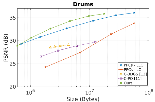
Fig. 3: RD results for “drums” in terms of PSNR (dB) vs the size (in Bytes) comparing our occlusion-aware compression scheme to PPC-based solutions, C-3DGS [13] and C-PO. [11]
