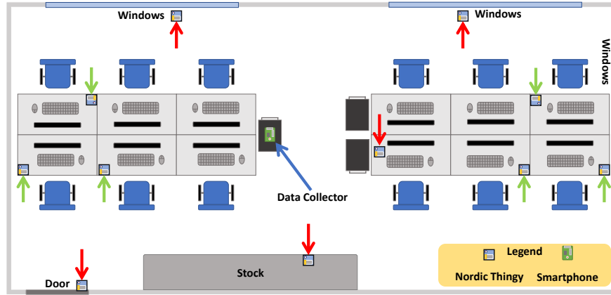
Fig. 5. Office 1.71. Motionless (red) and mobile (green) nodes and data collector (grey).
