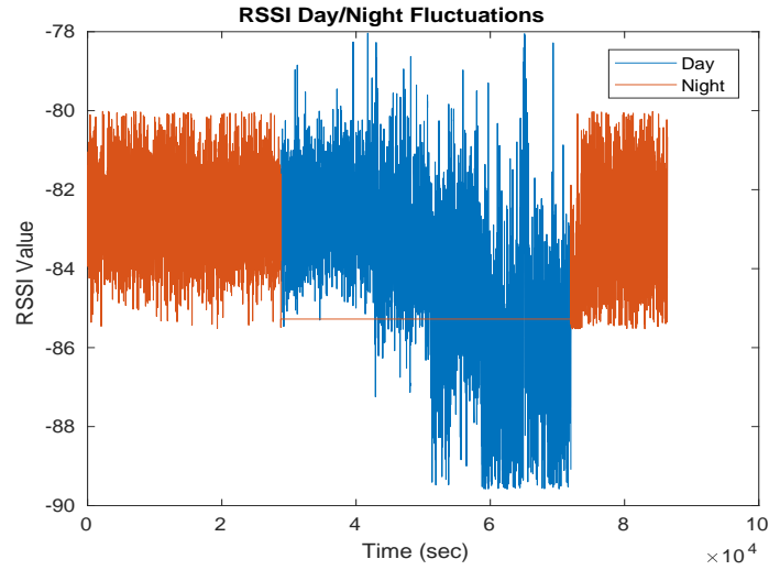
Fig. 6. Office 1.71. RSSI fluctuation between night and day for occupancy detection.
