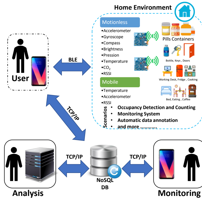
Fig. 2. Schematic view of the SHPIA platform.
