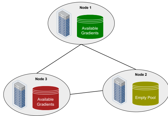
Figure 1: Illustration of delayed feedback in distributed system. Given a time t , each agent holds a distinct pool of available gradient feedback from s < t that is ready for computation at the current time. The pool can also be empty if no feedback is provided.
