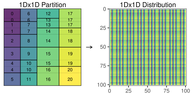
Figure 3: Left: the 1D-1D column-based partition; Right: after shuffling.
