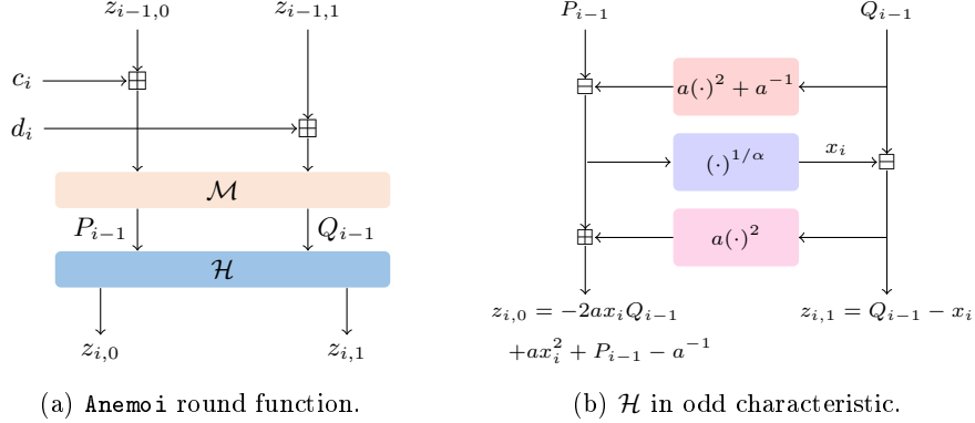
Fig. 4: Description of Anemoid over prime fields with \ell = 1 .
