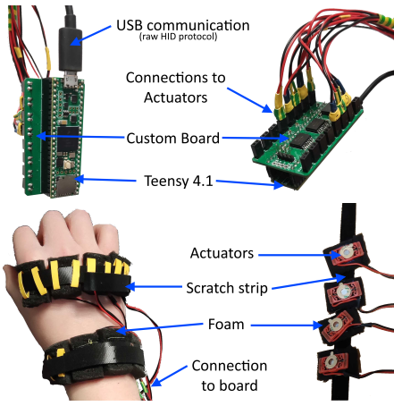
Figure 4: Apparatus used in the experiment. Left: Teensy 4.1 and custom boards. Right: actuators.
