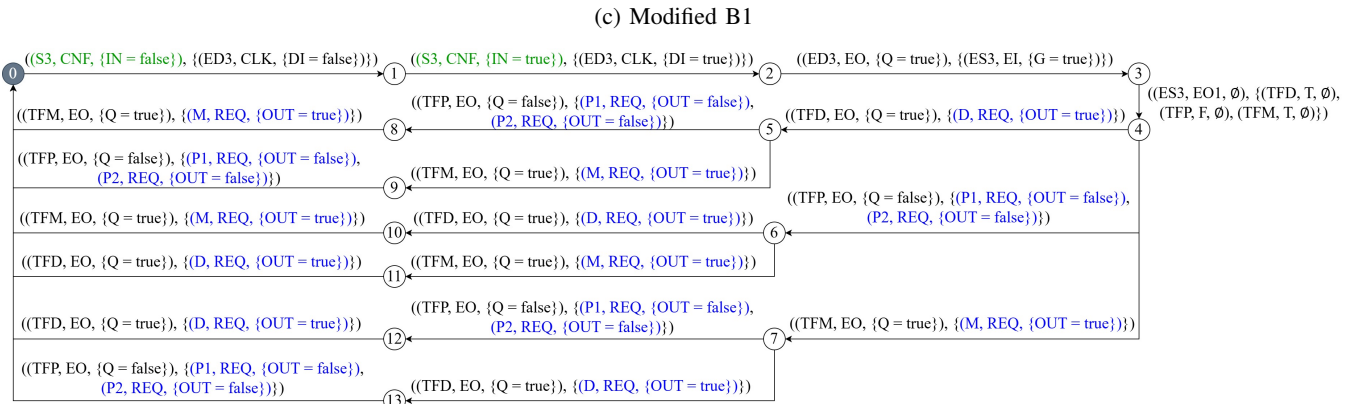
Fig. 10: Modified submodels
