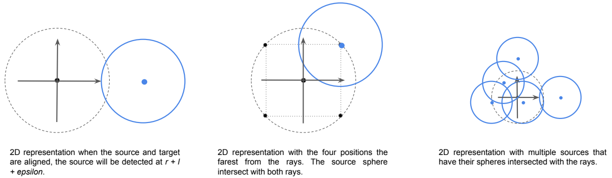
Figure 2: 2D Spherical representation of the particles in three different cases. In the first one (left), we show the position of the farthest source particle and how it will be detected by the ray. In the second one (center), we show the case where the source particle is the farthest from the rays (it also shows that in 2D the sphere radius could be smaller). In the last one (right), we show different source particles with their spheres and the rays that will intersect with them.
