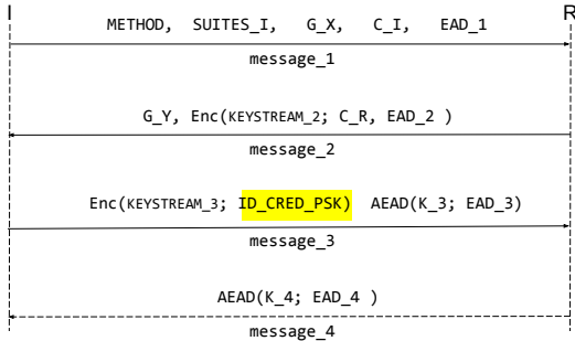
(b) Message flow of EDHOC with symmetric keys. Approach B.
