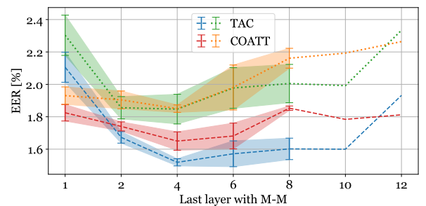
Figure 3: Performance dependence on the last layer where the M-M module is inserted (with the take-first downstream M-S). Red and blue colors correspond to MRE eval., green and orange to MRE_hard eval. Shaded areas depict standard deviations obtained on four runs.
