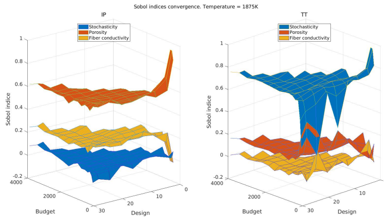
Figure 7: Convergence of Sobol indices when increasing C and N .
