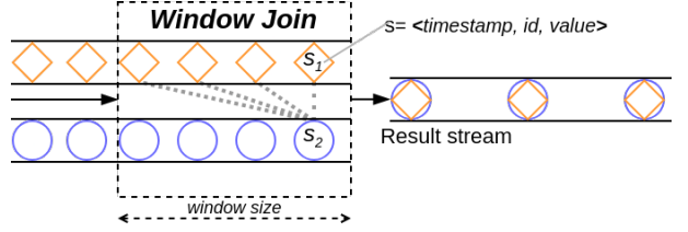
Fig. 3. Window join mechanisms.
