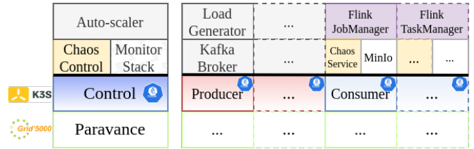
Fig. 1. Experimental platform.
