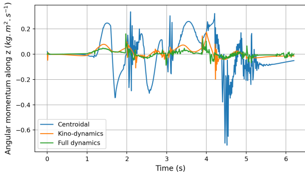
Fig. 7. Comparison of the vertical component of the angular momentum during stairstep climbing.
