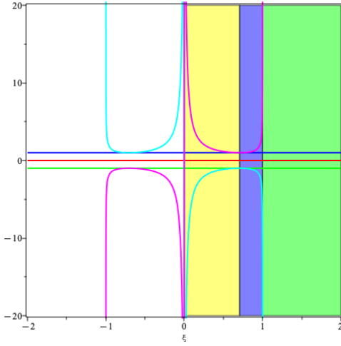
(a) The curves defined by \gamma \in \mathbb{Q}[\xi] corresponding to R \in \mathbb{Q}[\xi][\gamma] for \omega_n = 1 .
