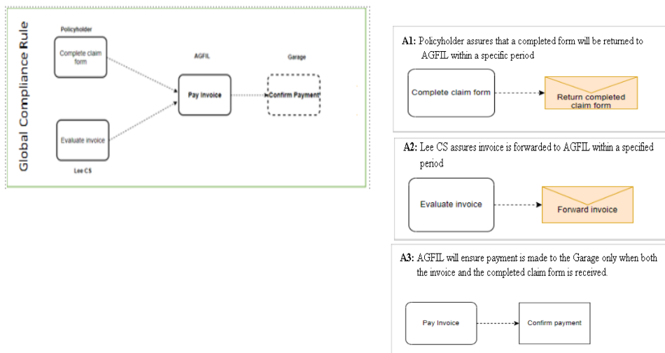
Fig 3. GCR 1 and its Assertion
