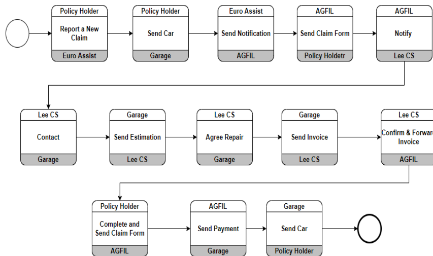
Fig. 2. Choreography Model for Insurance Case
