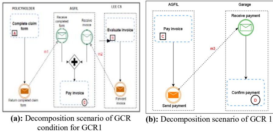
Fig. 4. Decomposition of GCR 1
