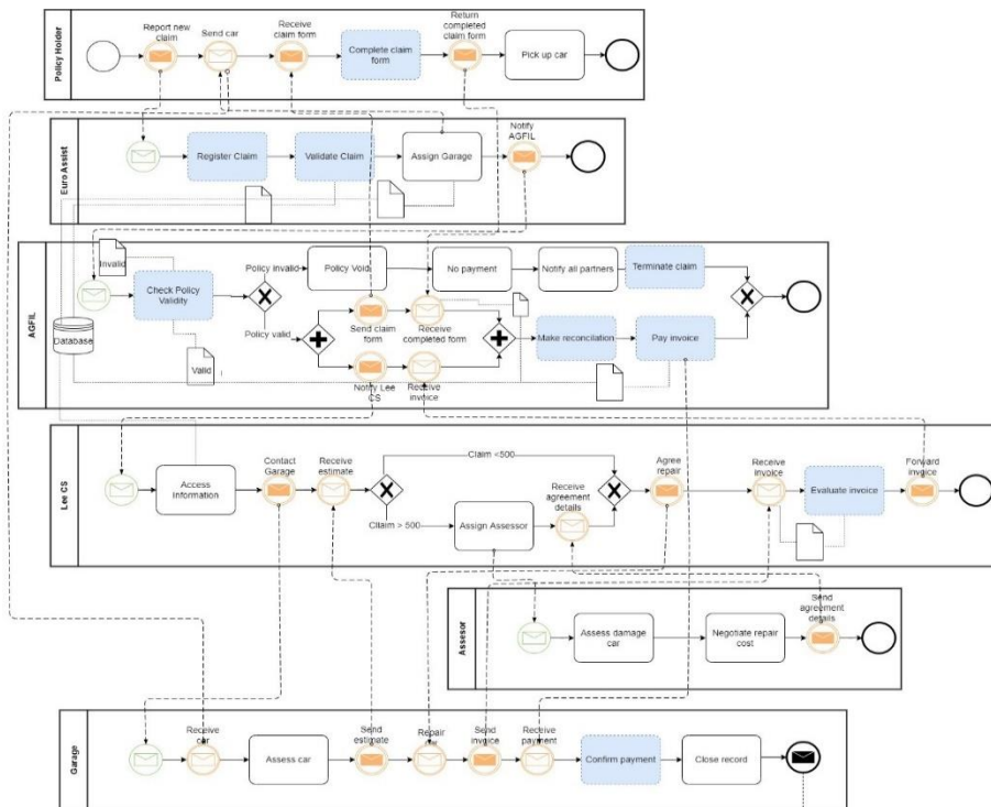
Fig. 1. Collaborative Model for Insurance Case [1] [2].
