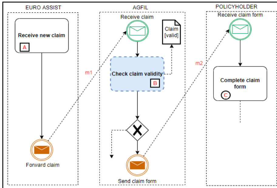
Fig 6. Decomposition scenario of GCR 2
