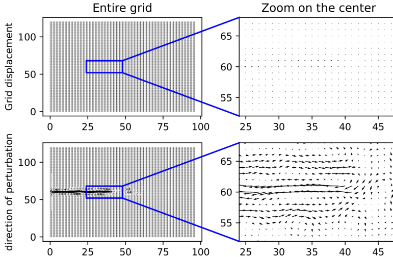
Figure 4. Visualization of the perturbation of the grid generated by the SGP method for one of the ensemble members at the end of a one-year simulation. Arrows linking the initial grid to the perturbed grid are plotted: the length of the arrows was multiplied tenfold in the bottom part to better visualise the direction of the perturbation. On the left, the whole grid is represented and the right panel is a zoom on a smaller portion.
