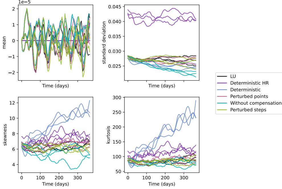
Figure 8. First four standardized moments of the variable u (reconstructed from p ). Only 3 ensemble members out of 30 are displayed for each ensemble to facilitate better visualization.
