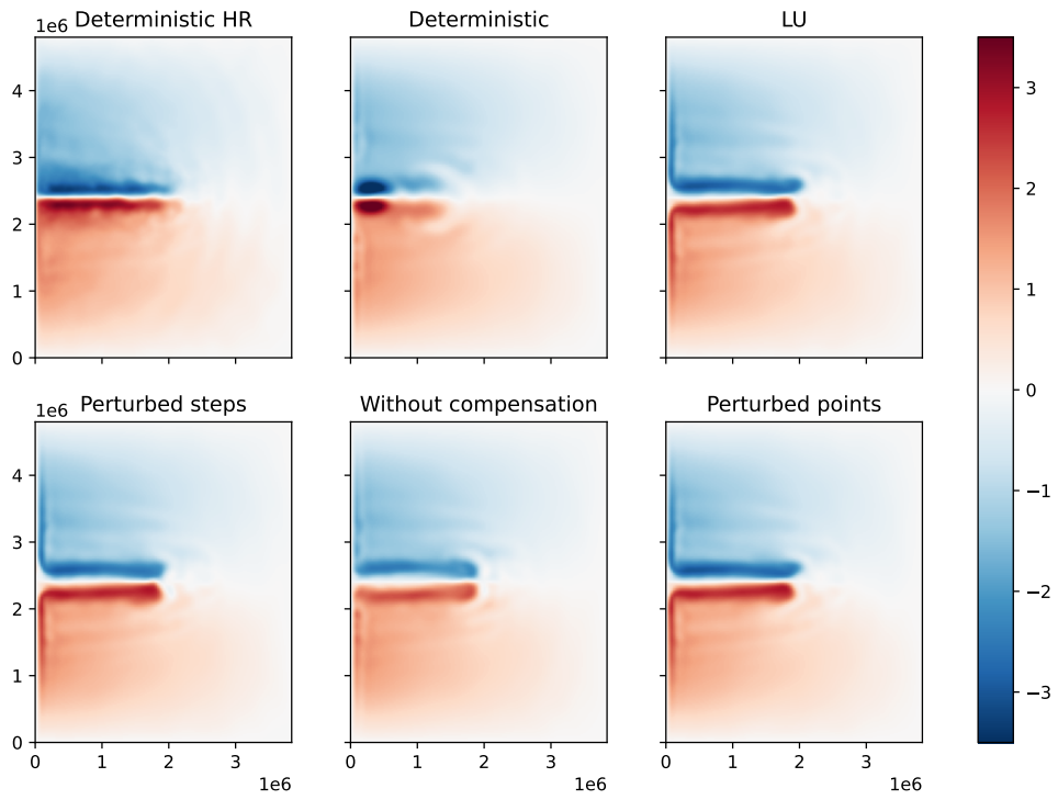
Figure 5. Surface pressure (in \text{m}^2 \cdot \text{s}^{-2} ) averaged over the last week of a one-year simulation.
