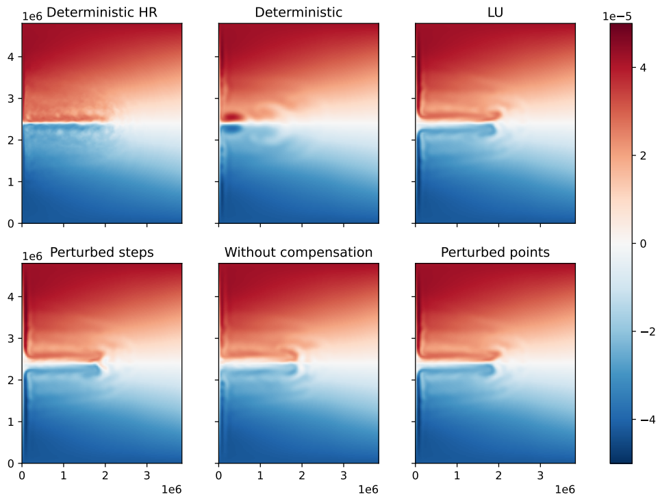
Figure 6. Surface potential vorticity (in \text{s}^{-1} ) averaged over the last week of a one-year simulation.
