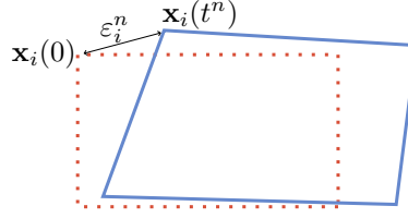
Figure 1. Illustration of the grid perturbation: dotted lines represent the initial grid and solid lines represent the perturbed grid at time t^n . All points are drifted to the right in order to illustrate the fact that the noise is spatially correlated.
