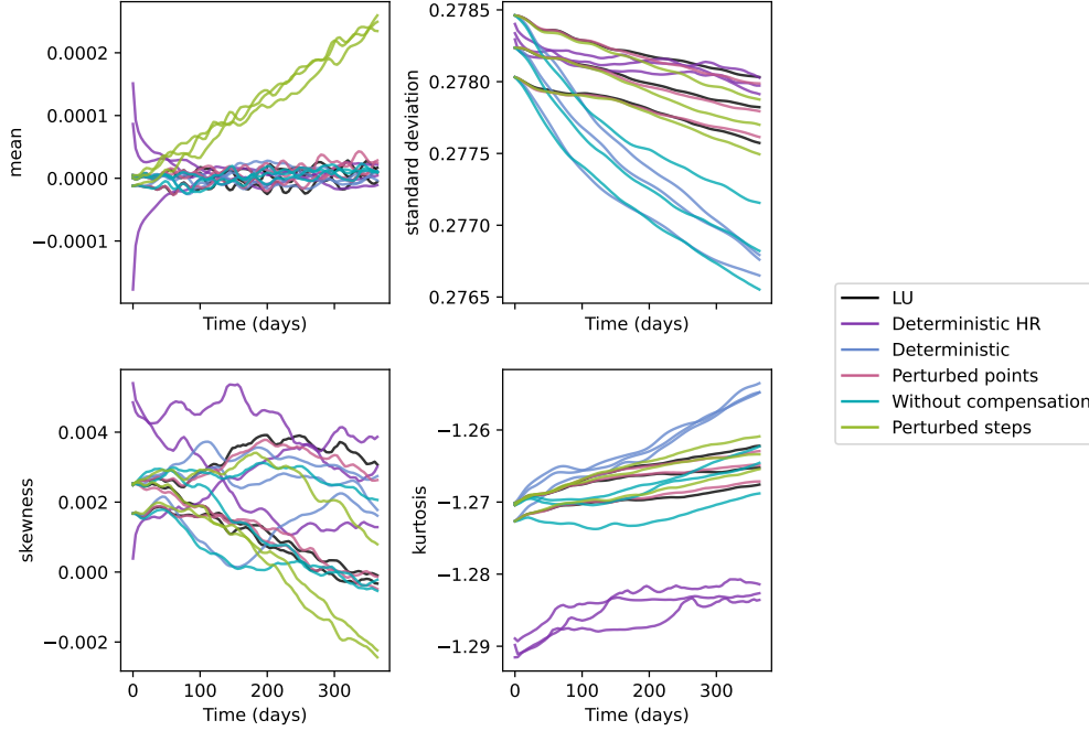
Figure 9. First four standardized moments of the variable q . As in Figure 8, only 3 ensemble members out of 30 are displayed for each ensemble simulation.
