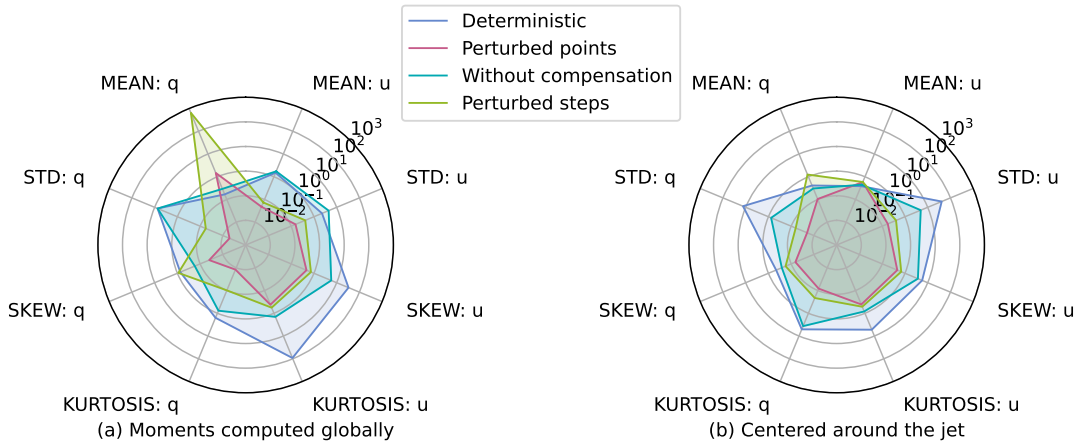
Figure 10. Log scaled radar chart showing the relative distance to LU for the first four standardized moments of the variables u and q . Left panel (a): summary of Tables 2 and 3: the standardized moments are computed on the whole computational domain. Right panel (b): additional analysis where the standardized moments are computed on a smaller portion of the domain, including the jet area.
