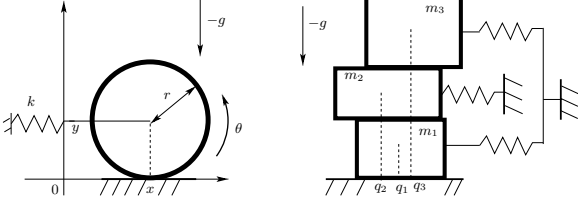
Fig. 1. Left: Sliding disc. Right: stacked blocks.
