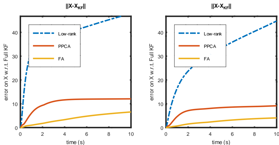
Figure 2: d = 200 with p = 8 (left) and p = 50 (right). Norm of the error over time between the filters' state estimates and the full KF's optimal estimate, for a randomly picked initial error in a noise-free setting.
