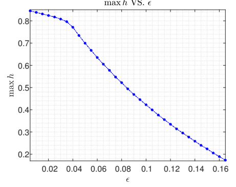
Fig. 1. Theorem 3.1 - max h which preserve feasibility of (3.18) and \delta_{2,x} < e^{-\alpha h} .
