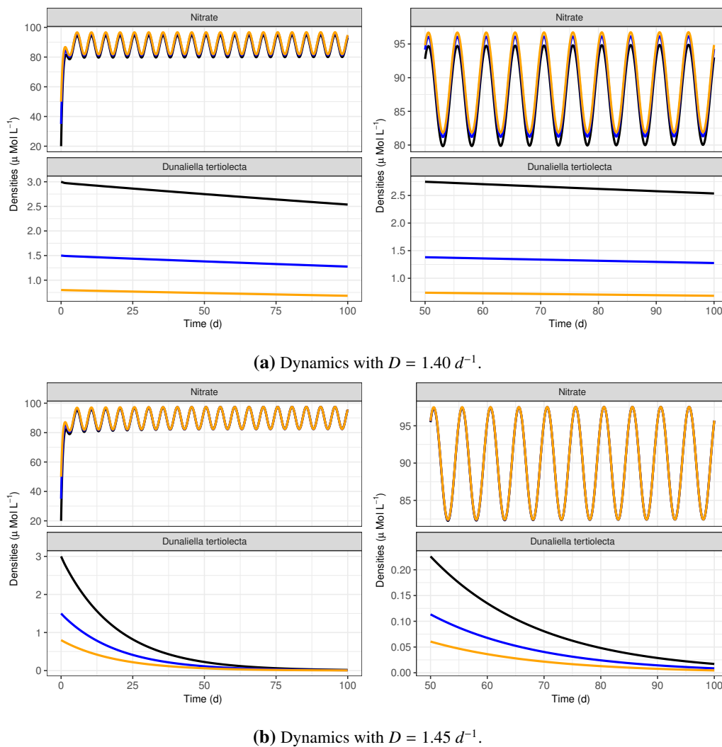
Figure 4. Dynamics of the total biomass and substrate. The initial conditions are: (s, x) = (20, 3) (black curve), (s, x) = (35, 1.5) (blue curve) and (s, x) = (50, 0.8) (orange curve).
