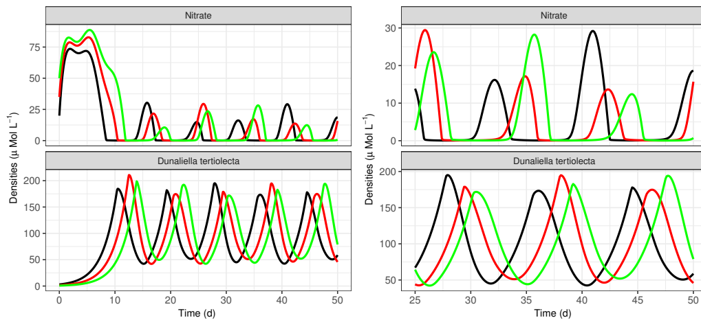
(c) Dynamics with \tau = 2.0 d .
