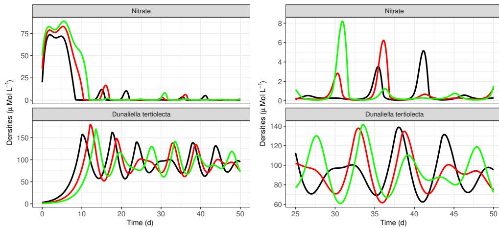
(a) Dynamics with \tau = 1.6 d .
