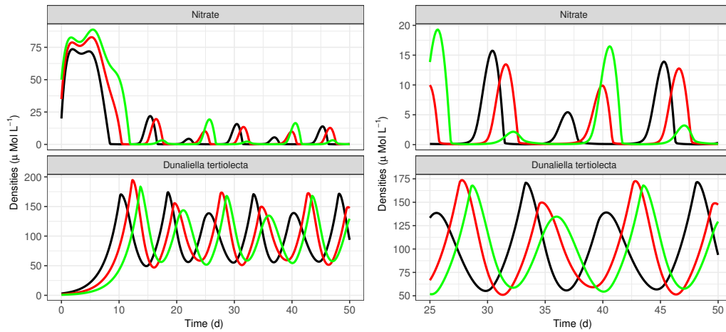
(b) Dynamics with \tau = 1.8 d .
