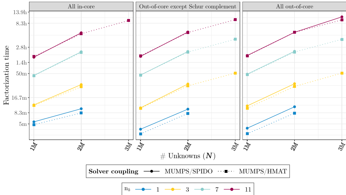
FIG. 20: Computation times of baseline multi-factorization and compressed Schur multi-factorization on coupled FEM/BEM linear systems of varying number of unknowns and for varying values of n_b . We test 3 different configurations of the out-of-core feature: completely disabled, enabled except for the Schur complement matrix or enabled including for the Schur complement matrix. Parallel runs on single bora node.
