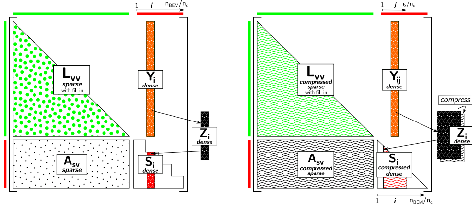
FIG. 3: Block-wise computation of S using the baseline multi-solve (left) and the compressed Schur multi-solve (right) algorithms.
