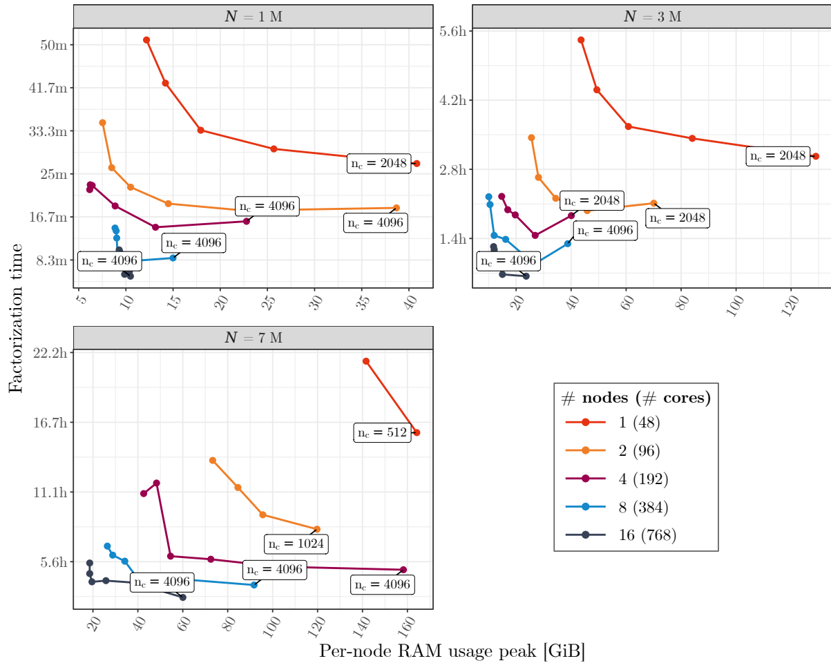
FIG. 13: Computation times of multi-solve with MUMPS/SPIDO on FEM/BEM linear systems of varying size N and for varying values of n_c . Labels indicate the highest achieved n_c . Parallel runs on 1 to 16 skylake nodes (48 threads/node).
