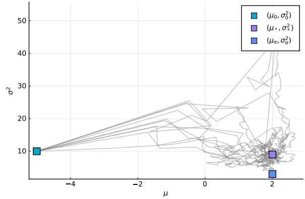
(b) Plot of 10 trajectories of Algorithm 7, with the point (\mu_*, \sigma_*^2) to which the trajectories converge and the point (\mu_\pi, \sigma_\pi^2) encoding the distribution of the samples.
