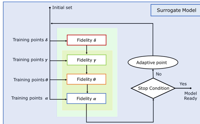
FIG. 4: Sketch of the multi-fidelity adaptive surrogate model construction.
