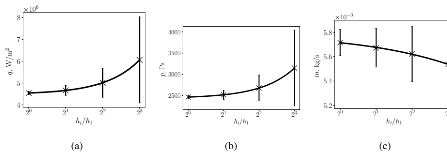
FIG. 11: Grid convergence study for the (a) stagnation-point heat flux, (b) stagnation-point pressure, and (c) nozzle mass flow rate. Cross: CFD value; solid line: fit law according to Eq. (18); bars: numerical uncertainty according to Eq. (19).
