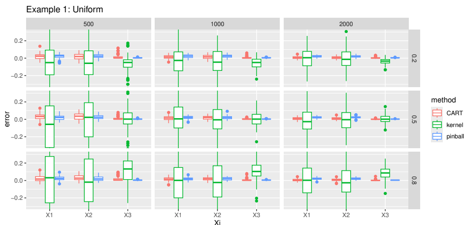
Figure 3: Estimation error for Example 1, at different quantile levels (0.2, 0.5, 0.8) and for different sample size (500, 1000, 2000).
