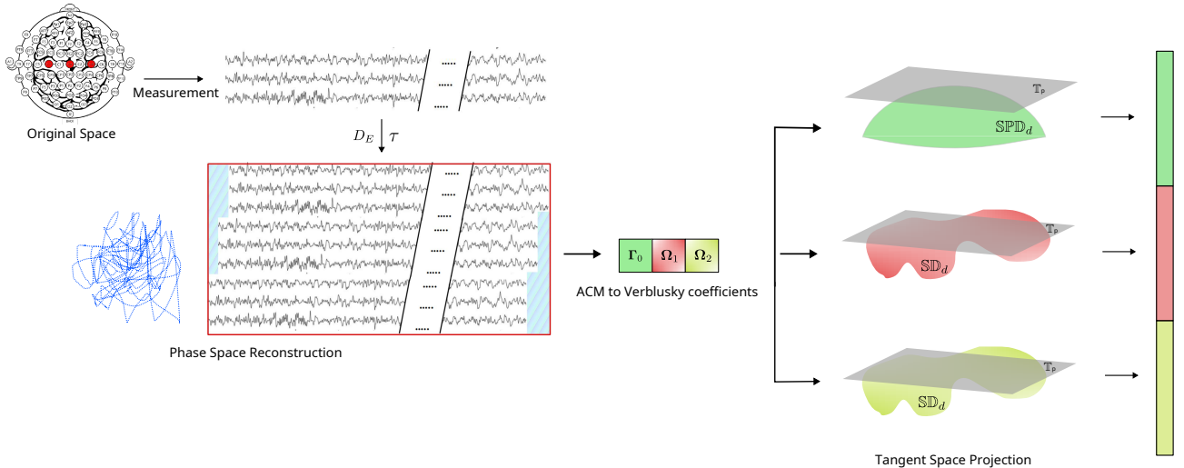
Figure 1: Schematic illustration of the BT-ACM + TG + SVM methodology. The presented example uses only 3 electrodes (in red on the top left plot). The measurement process of the original dynamic system is thus a 3-dimensional time series. The process then begins with the extraction of epoch signal representing left and right hand tasks. We then use the phase space reconstruction process to obtain a dynamic system equivalent to the original one (selection of hyper-parameters are made via grid search using the nested approach). In this figure, we see an embedding corresponding to p = 3 and \tau = 10 . The BT-ACM matrix is computed as the autocovariance of this high-dimensional time series. Subsequently the main blocks are converted in Verblunsky coefficients. Then, each component is mapped to the tangent space using the appropriate Riemannian manifold computations and vectorized. The final step is the application of an SVM-based classification algorithm.
