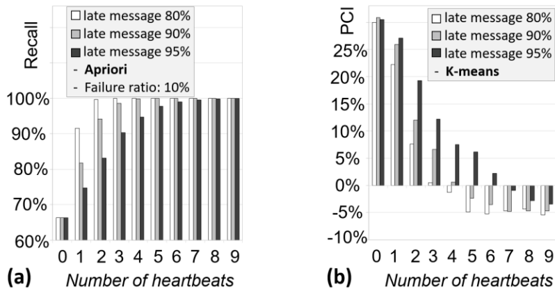
Figure 19: Heartbeat Execution Quality (Apriori and K-means)
