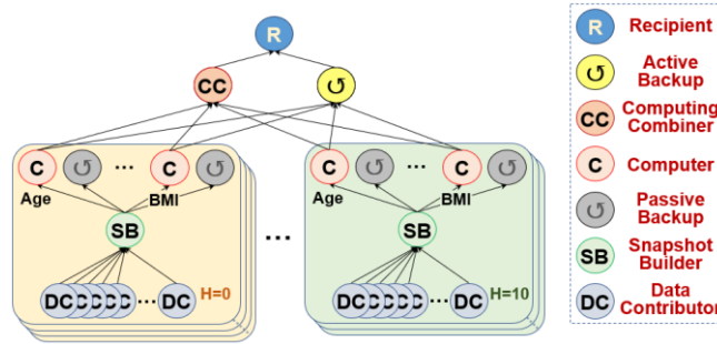
Figure 9: Hybrid-based Strategy
