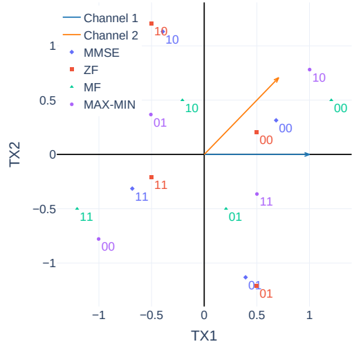
Fig. 1: Constellation of the different encoders with non-orthogonal channels
