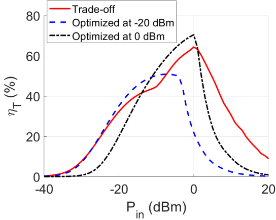
Fig. 11. Simulated efficiency comparison of a rectifier optimized at -20 dBm, 0 dBm and the rectifier association optimized at -20 dBm and 0 dBm.
