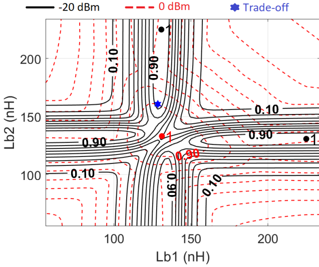
Fig. 10. Evaluation of L_{b1} and L_{b2} to obtain high efficiencies at -20 dBm and 0 dBm. Contours indicate normalized simulated efficiencies \eta_T .
