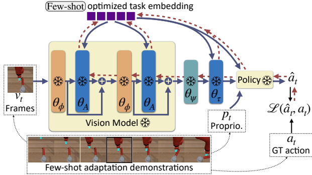
(b) Optimization of the task embedding in the Few-shot setting.
