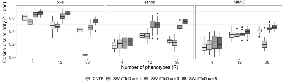
Fig. 11 Cosine dissimilarity between pairs of sets of phenotypes with respect to the phenotypes’ size for SWoTTED, and CNTF. The lower the dissimilarity, the more similar are the sets of phenotypes between each run.
