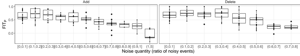
Fig. 10 FIT_P values of SWoTTED on synthetic data as a function of normalized noise (% of new or deleted events).
