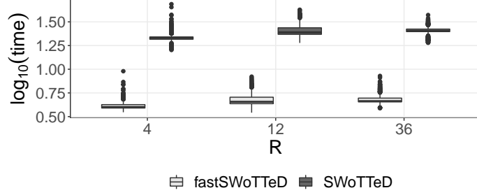
Fig. 17 \log_{10}(\text{time}) (in seconds) for training SWoTTED and FASTSWoTTED models.
