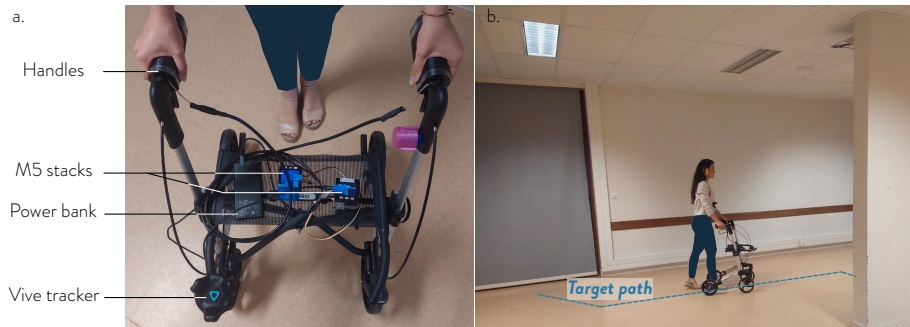
Fig. 2. a) Experimental setup: The handles are mounted on the walker. Signals are amplified and sent to the handles by the M5 Stacks controllers connected via WiFi. The motors are powered through the M5 Stacks cabled to a power bank. b) Navigation: The participant is guided by the tactile patterns along a target virtual path (not visible by the user, dashed blue line in the Figure).
