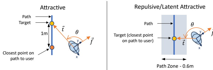
Fig. 2. Each navigation strategy (Attractive A, Repulsive R, Latent Attractive LA) computes a signed angle \theta between the user heading direction \vec{f} and a vector pointing toward a target on path \vec{t} . The Attractive strategy sets the target as the point on the path one meter ahead from the closest point on path to the user. The Repulsive and Latent strategies set the target to the closest point on path to the user.
