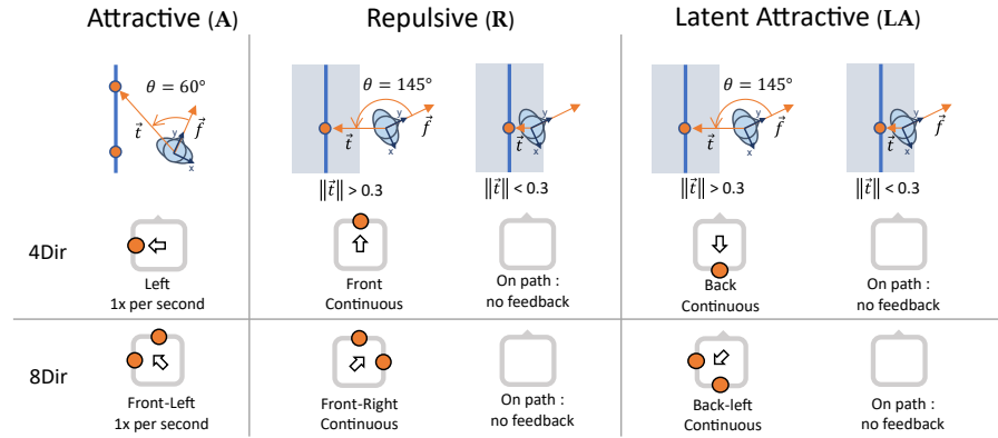
Fig. 4. Navigation strategies (Attractive A, Repulsive R, Latent Attractive LA) are combined with the two rendering schemes (4Dir, 8Dir). The orange circles (bottom) represent the actuators which are activated on the handle, depending on the position and orientation of the user relative to the path (top).
