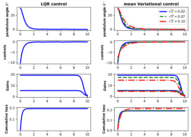
Fig. 2. Linearized LQR at equilibrium versus our ‘‘variational control’’ for the inverted pendulum regulation where we apply for the KL the mean policy \mathbb{E}[u_k|x_k] for different values of entropic regulation \sqrt{\varepsilon} = 0.02, 0.07, 0.10 . From the top to the bottom row, we show the angle \theta converted in degrees, the control, the two gains for angle and angular velocity, and finally, we compare both LQR and variational control with the same LQR quadratic loss.
