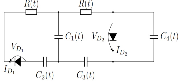
Figure 1: Time-varying RC circuit with ideal diodes.
