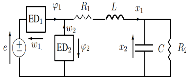
Figure 2: Circuit scheme of a DC/DC buck converter [1, Fig. 11].
