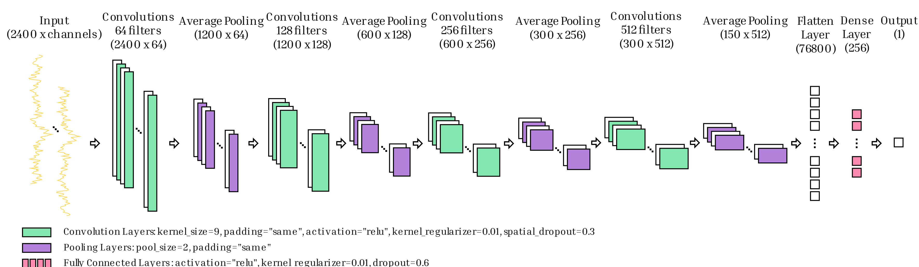
Fig. 1: Architecture of the 1D CNN used to predict fMRI NF scores from raw EEG signals. The input sample consists of 2400 timesteps from 25 EEG channels selected above the motor area.
