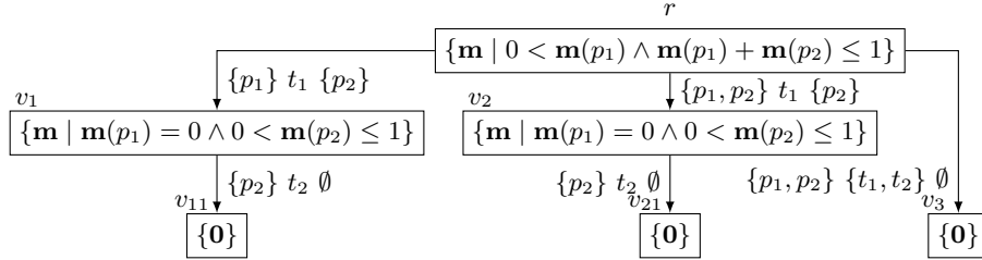
Fig. 4. The symbolic reachability tree of the marked CPN of Figure 2.
