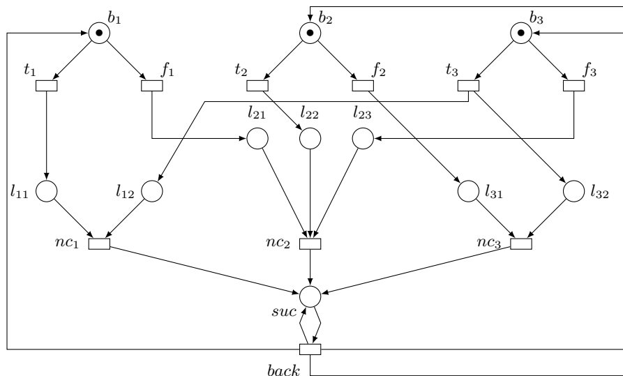
Fig. 6. The CPN corresponding to formula (\neg x_1 \vee \neg x_3) \wedge (x_1 \vee \neg x_2 \vee x_3) \wedge (x_2 \vee \neg x_3) .
